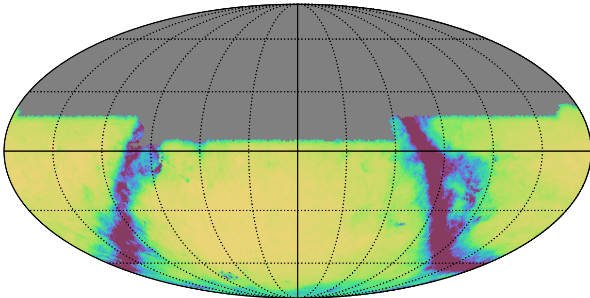
extra_ss_neo3_v3.4_10yrs All sky u band: Exgal_CoaddM5
