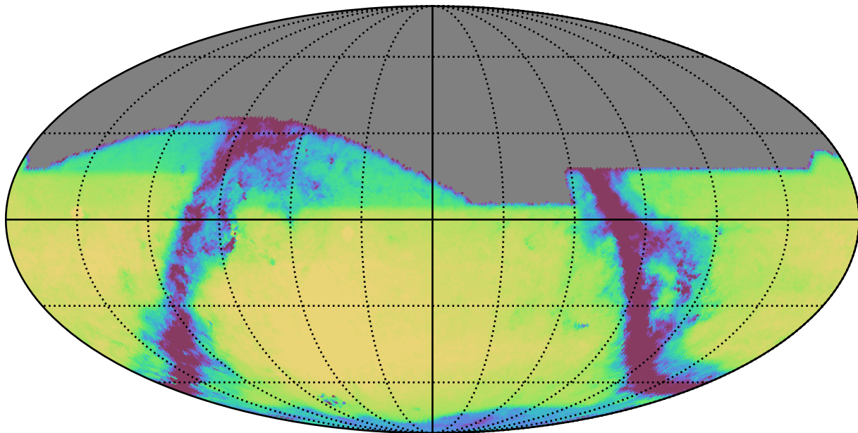
extra_ss_neo3_v3.4_10yrs All sky r band: Exgal_CoaddM5
