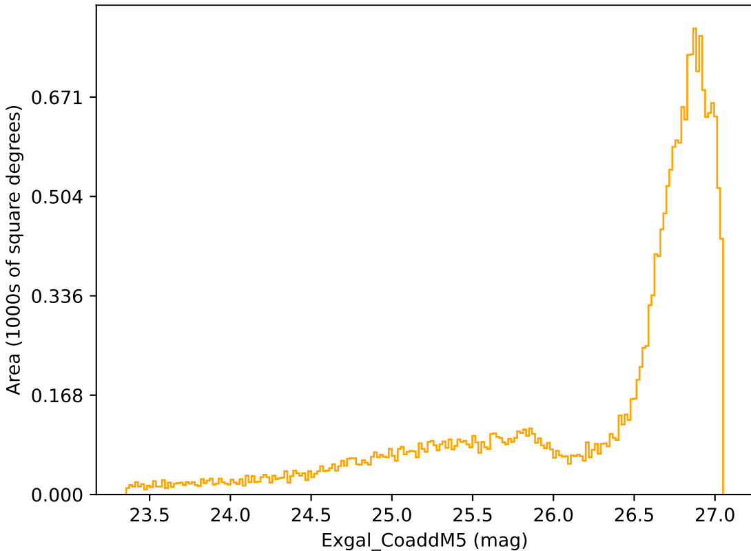
extra_ss_neo3_v3.4_10yrs All sky r band: Exgal_CoaddM5
