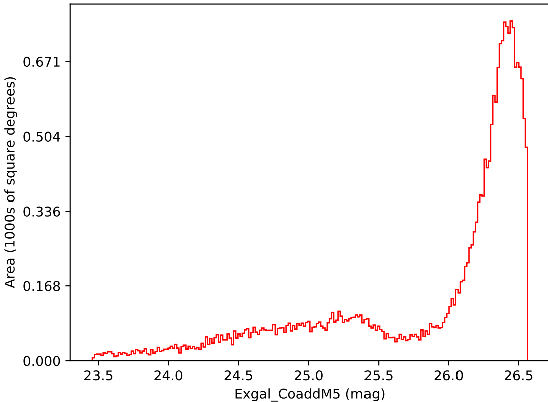
extra_ss_neo3_v3.4_10yrs All sky i band: Exgal_CoaddM5
