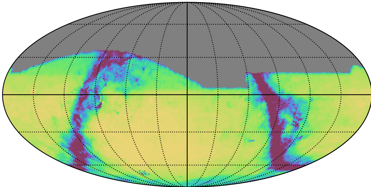
extra_ss_neo3_v3.4_10yrs All sky g band: Exgal_CoaddM5
