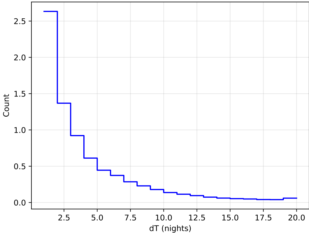
extra_ss_neo3_v3.4_10yrs WFD all bands: DeltaNight Histogram 1e6
