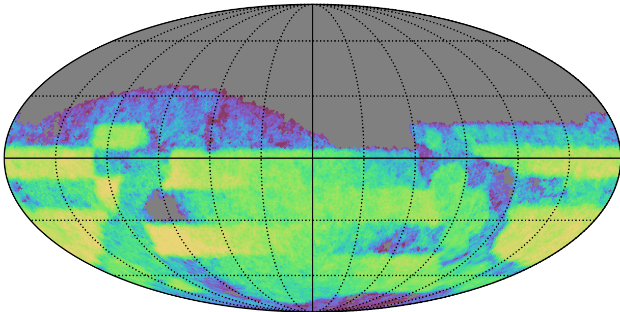
extra_ss_neo3_v3.4_10yrs Yr 3-4 z band: CoaddM5
