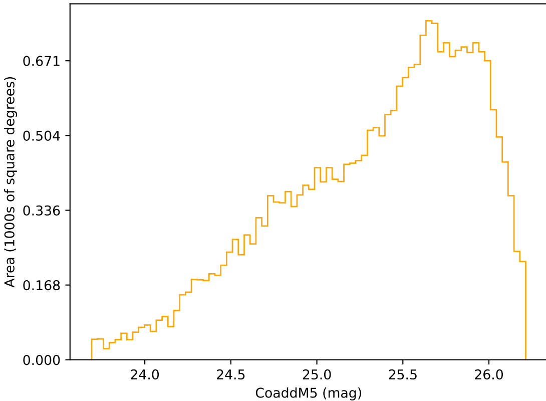
extra_ss_neo3_v3.4_10yrs Yr 3-4 r band: CoaddM5
