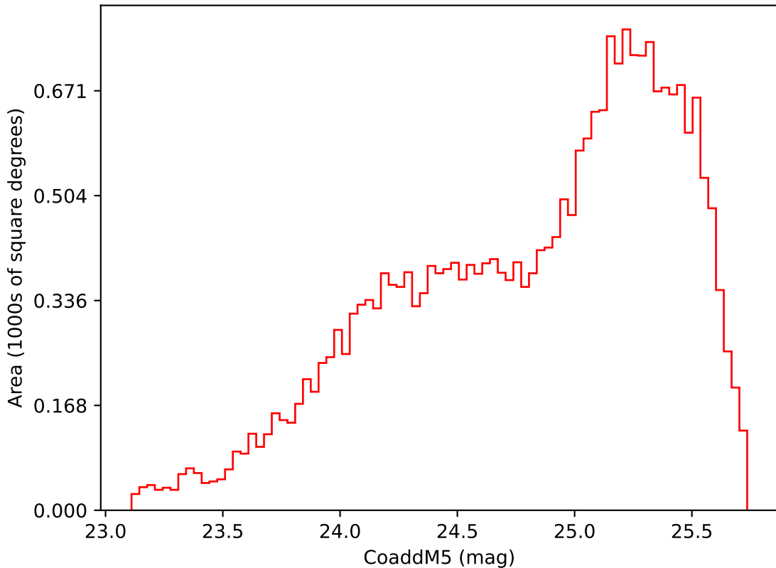
extra_ss_neo3_v3.4_10yrs Yr 3-4 i band: CoaddM5
