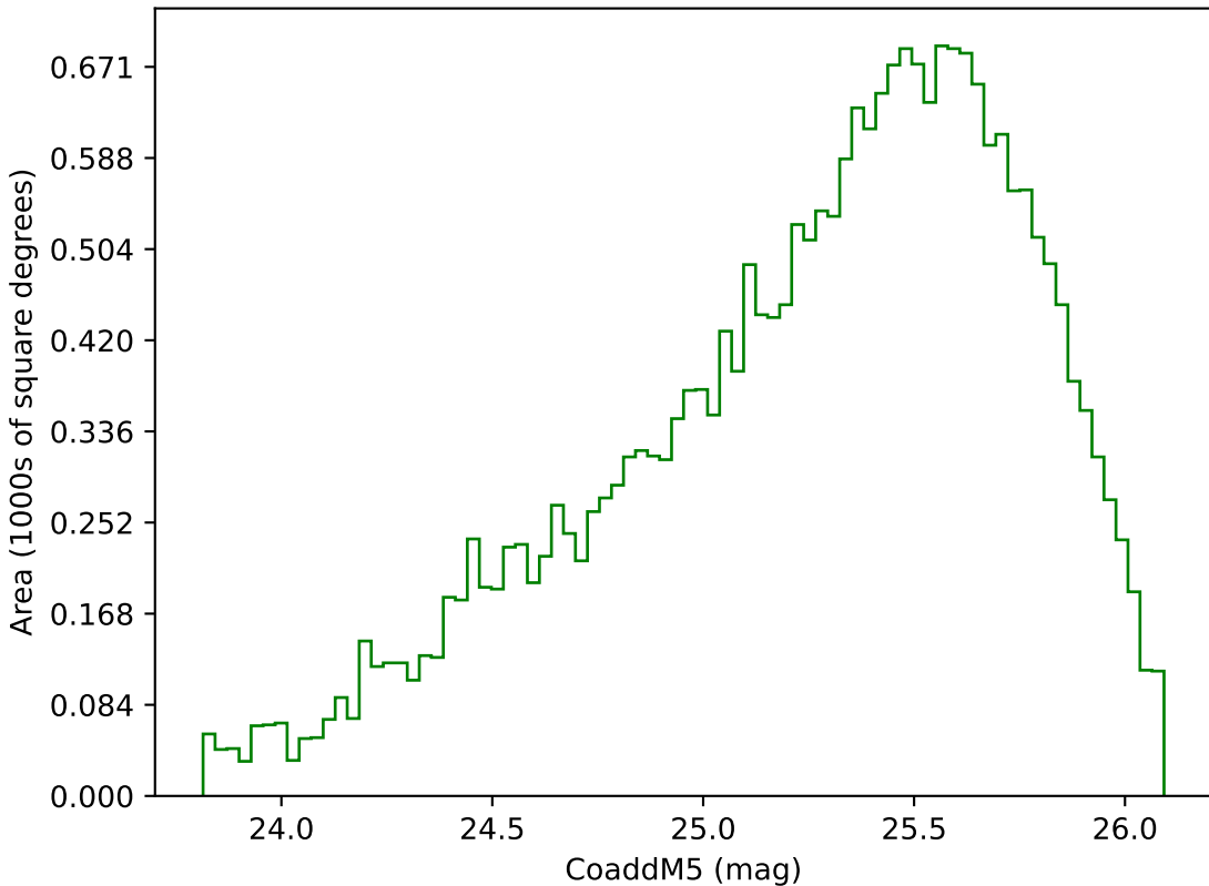
extra_ss_neo3_v3.4_10yrs Yr 3-4 g band: CoaddM5
