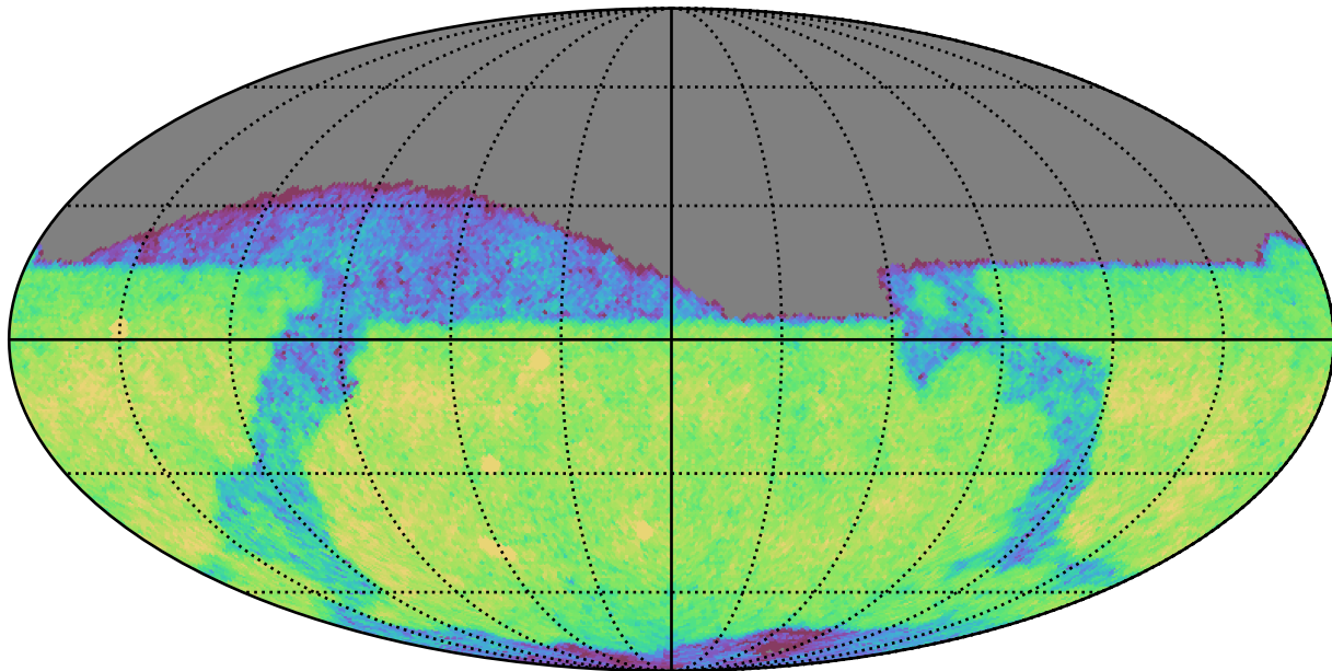
extra_ss_neo3_v3.4_10yrs Yr 1 z band: CoaddM5
