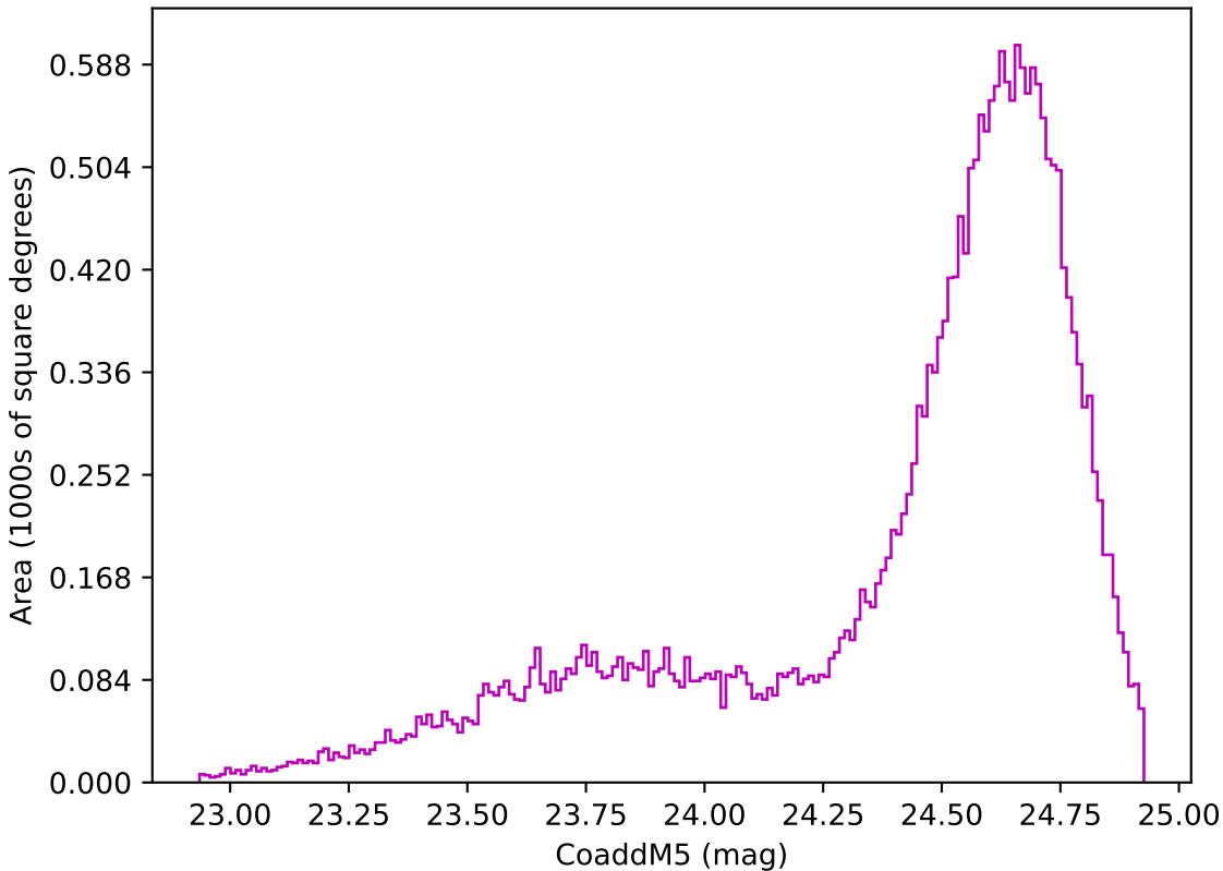
extra_ss_neo3_v3.4_10yrs Yr 1 z band: CoaddM5
