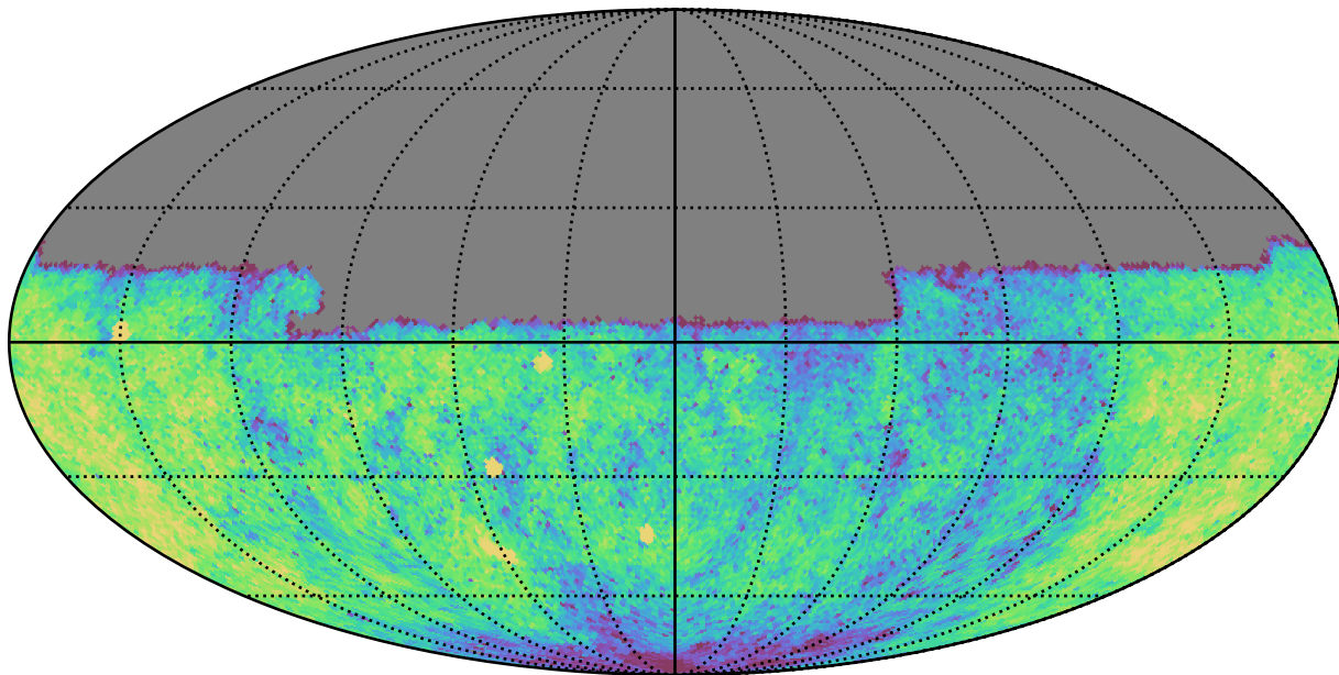
extra_ss_neo3_v3.4_10yrs Yr 1 u band: CoaddM5
