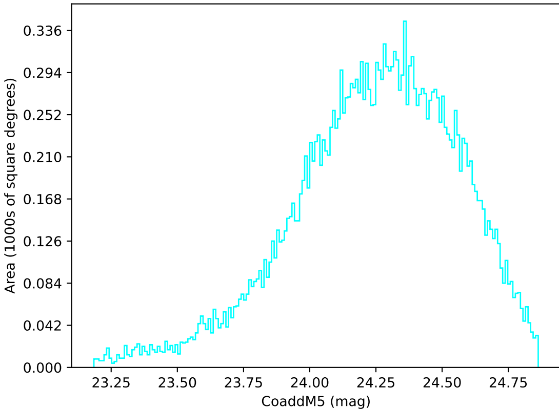
extra_ss_neo3_v3.4_10yrs Yr 1 u band: CoaddM5
