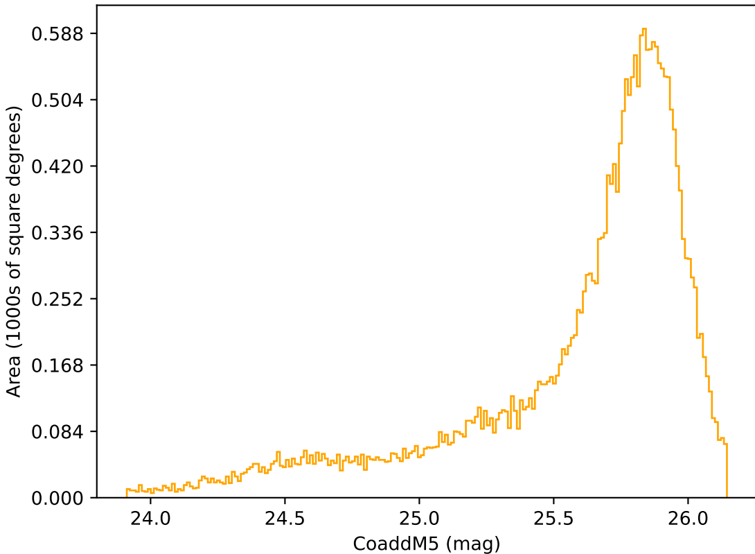
extra_ss_neo3_v3.4_10yrs Yr 1 r band: CoaddM5
