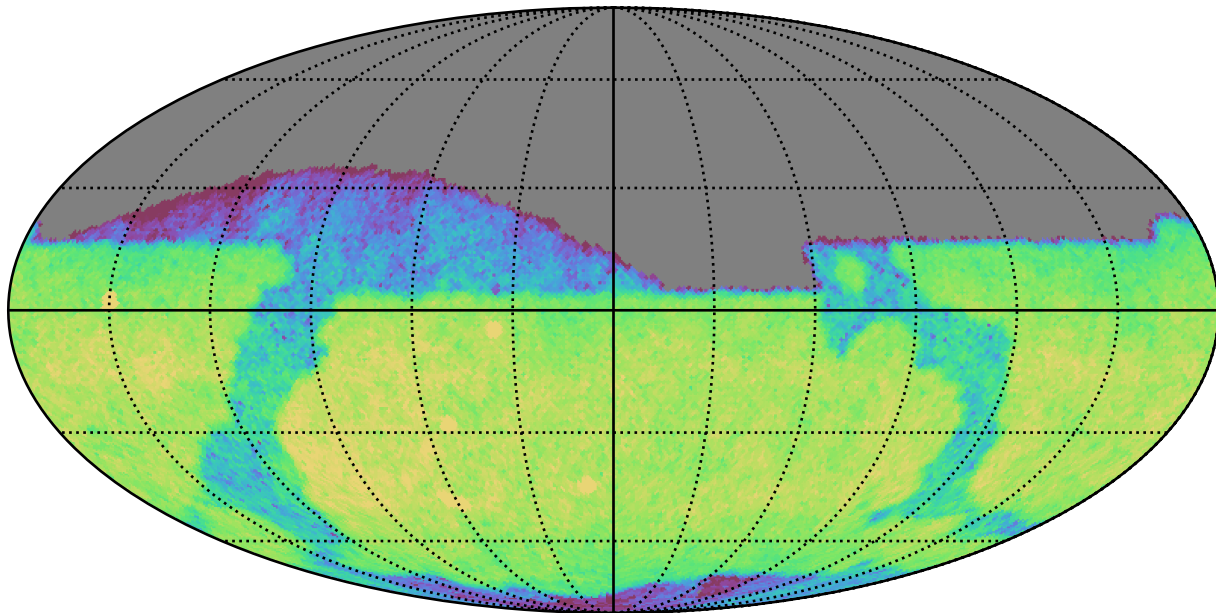
extra_ss_neo3_v3.4_10yrs Yr 1 i band: CoaddM5
