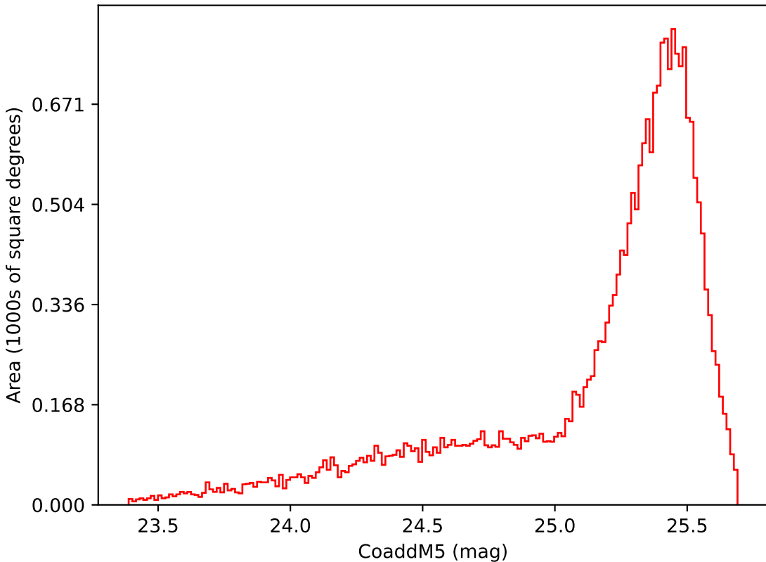
extra_ss_neo3_v3.4_10yrs Yr 1 i band: CoaddM5
