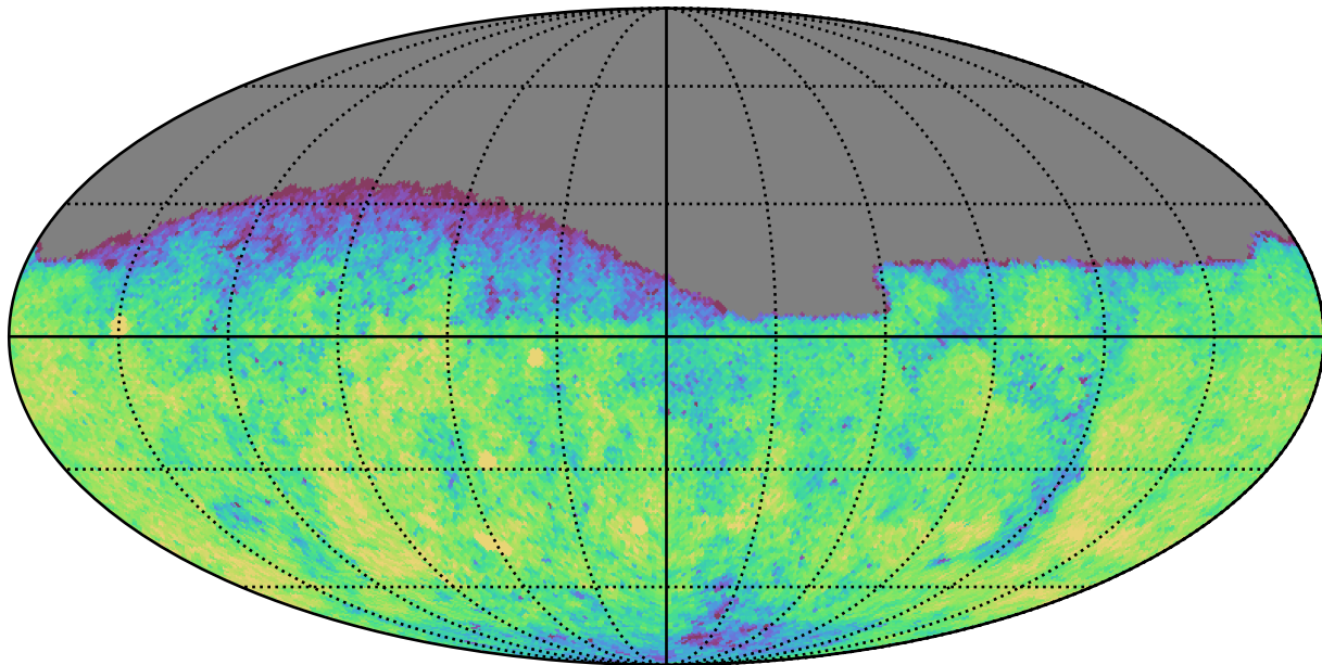
extra_ss_neo3_v3.4_10yrs Yr 1 g band: CoaddM5
