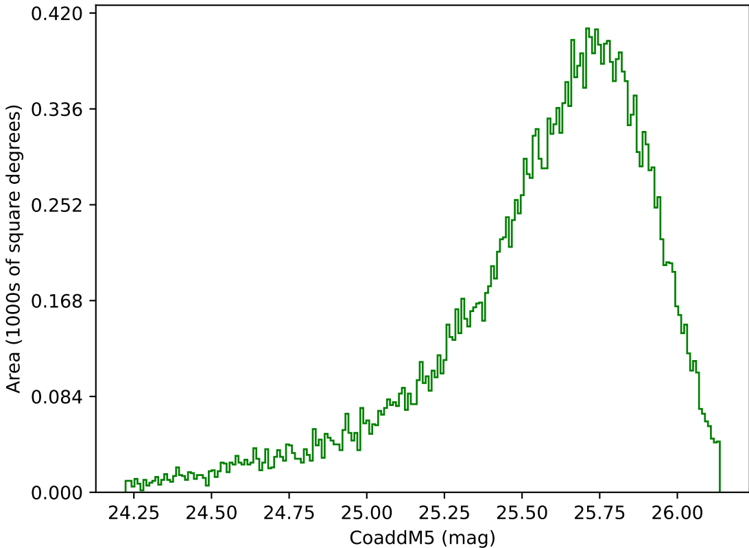
extra_ss_neo3_v3.4_10yrs Yr 1 g band: CoaddM5
