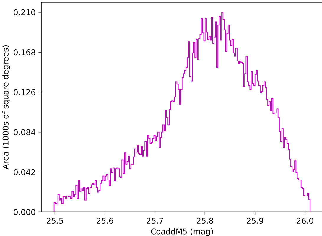
extra_ss_neo3_v3.4_10yrs WFD z band: CoaddM5
