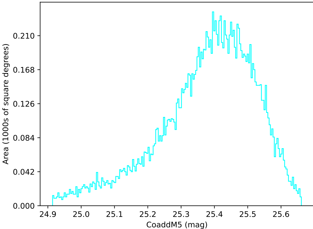
extra_ss_neo3_v3.4_10yrs WFD u band: CoaddM5
