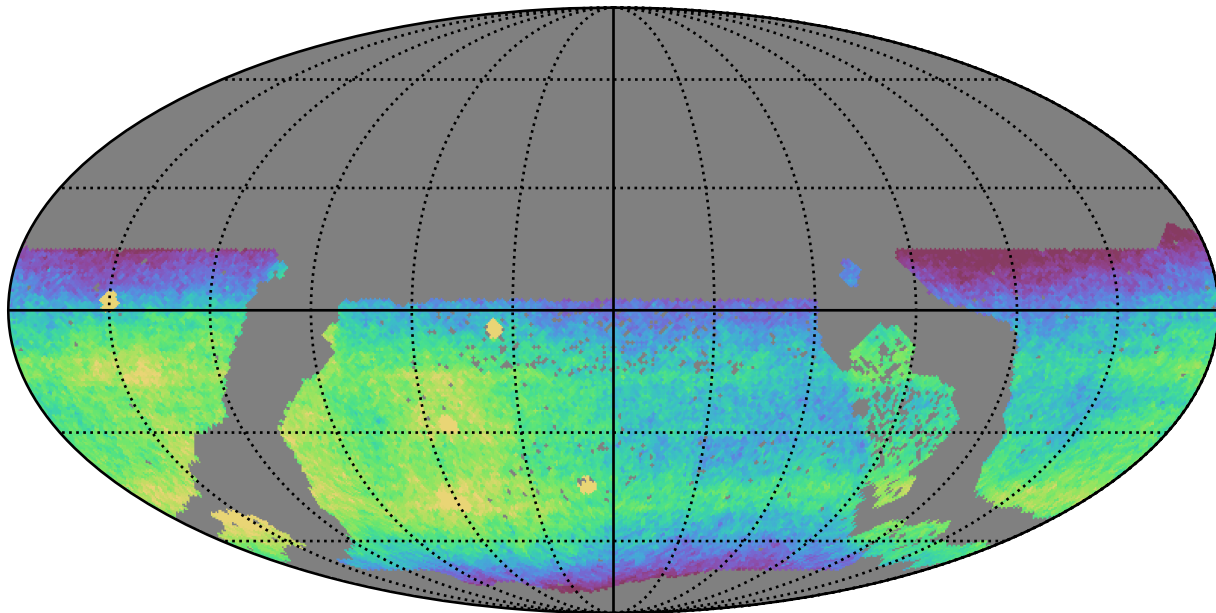
extra_ss_neo3_v3.4_10yrs WFD r band: CoaddM5
