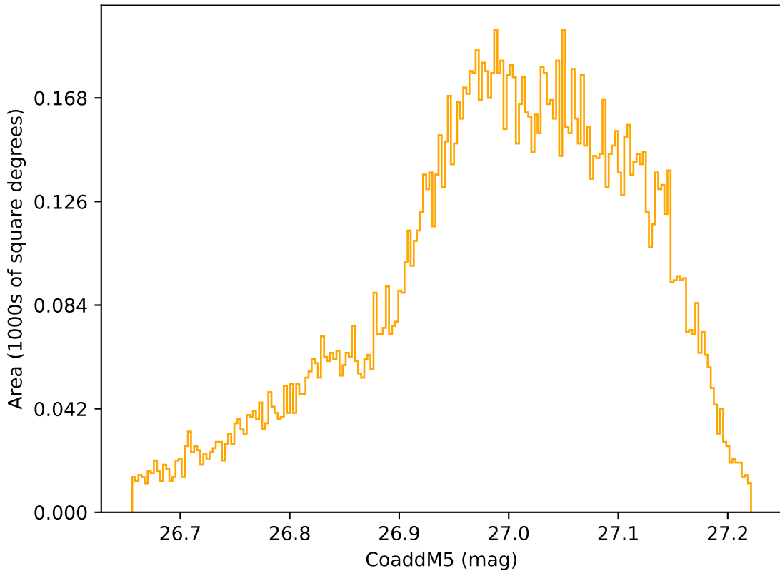
extra_ss_neo3_v3.4_10yrs WFD r band: CoaddM5
