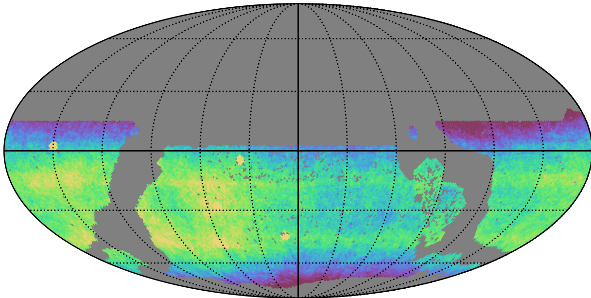
extra_ss_neo3_v3.4_10yrs WFD i band: CoaddM5
