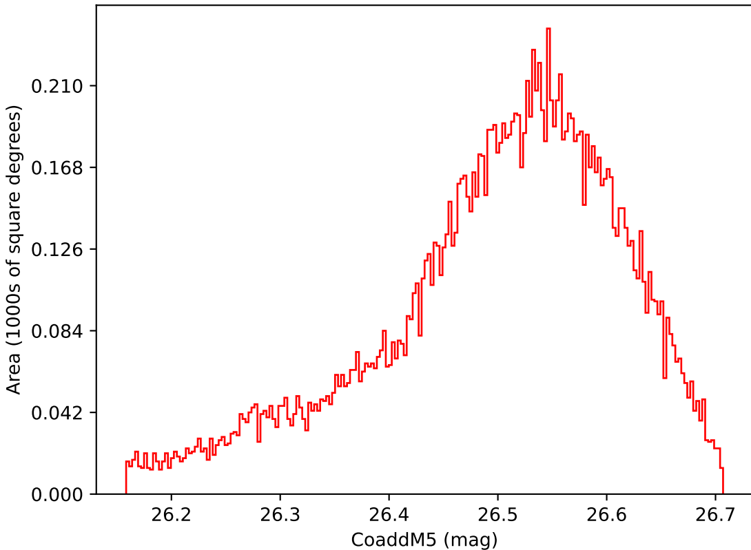
extra_ss_neo3_v3.4_10yrs WFD i band: CoaddM5
