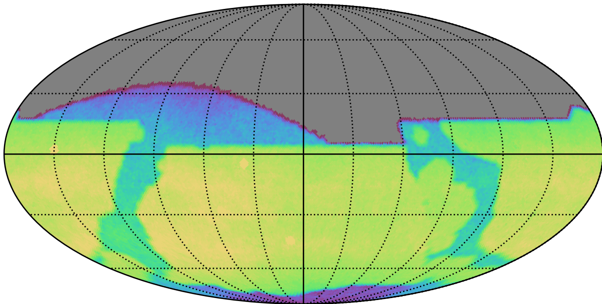
extra_ss_neo3_v3.4_10yrs All sky z band: CoaddM5
