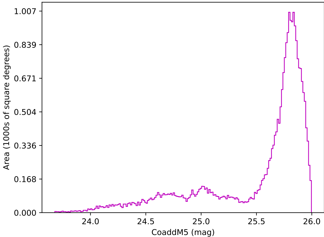
extra_ss_neo3_v3.4_10yrs All sky z band: CoaddM5
