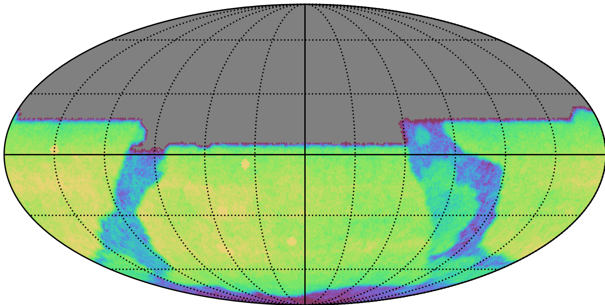
extra_ss_neo3_v3.4_10yrs All sky u band: CoaddM5
