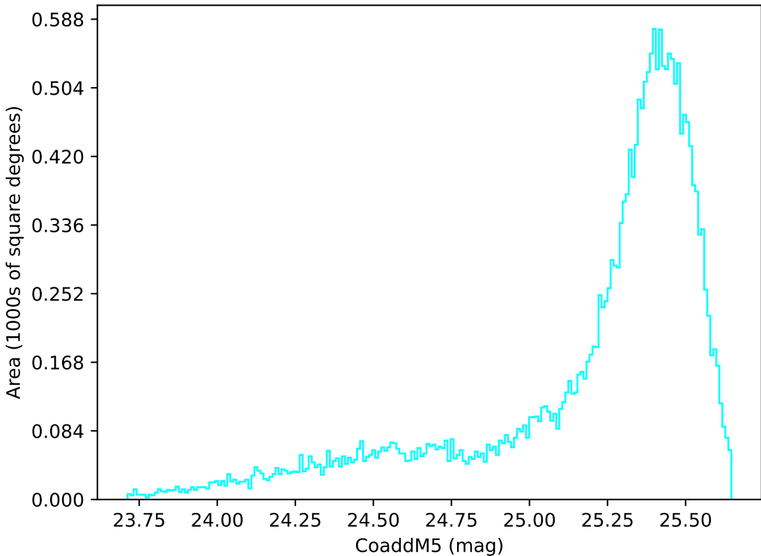
extra_ss_neo3_v3.4_10yrs All sky u band: CoaddM5
