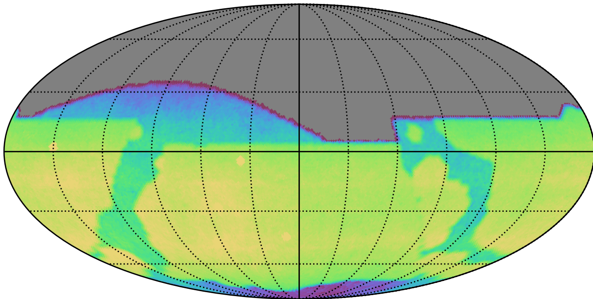
extra_ss_neo3_v3.4_10yrs All sky r band: CoaddM5
