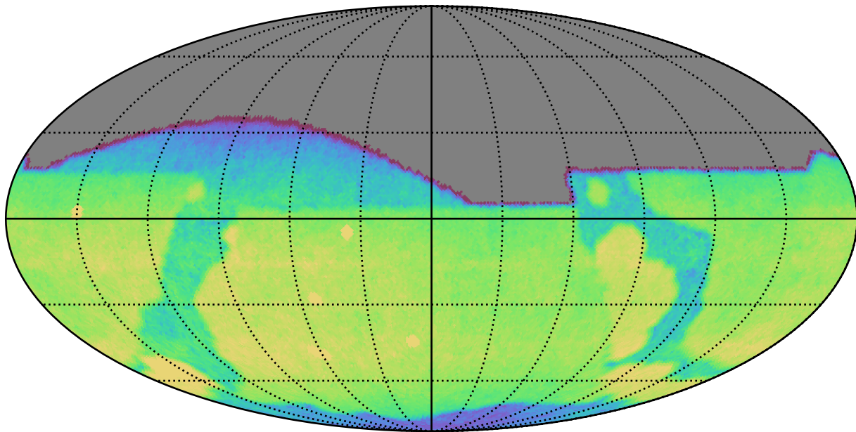
extra_ss_neo3_v3.4_10yrs All sky g band: CoaddM5
