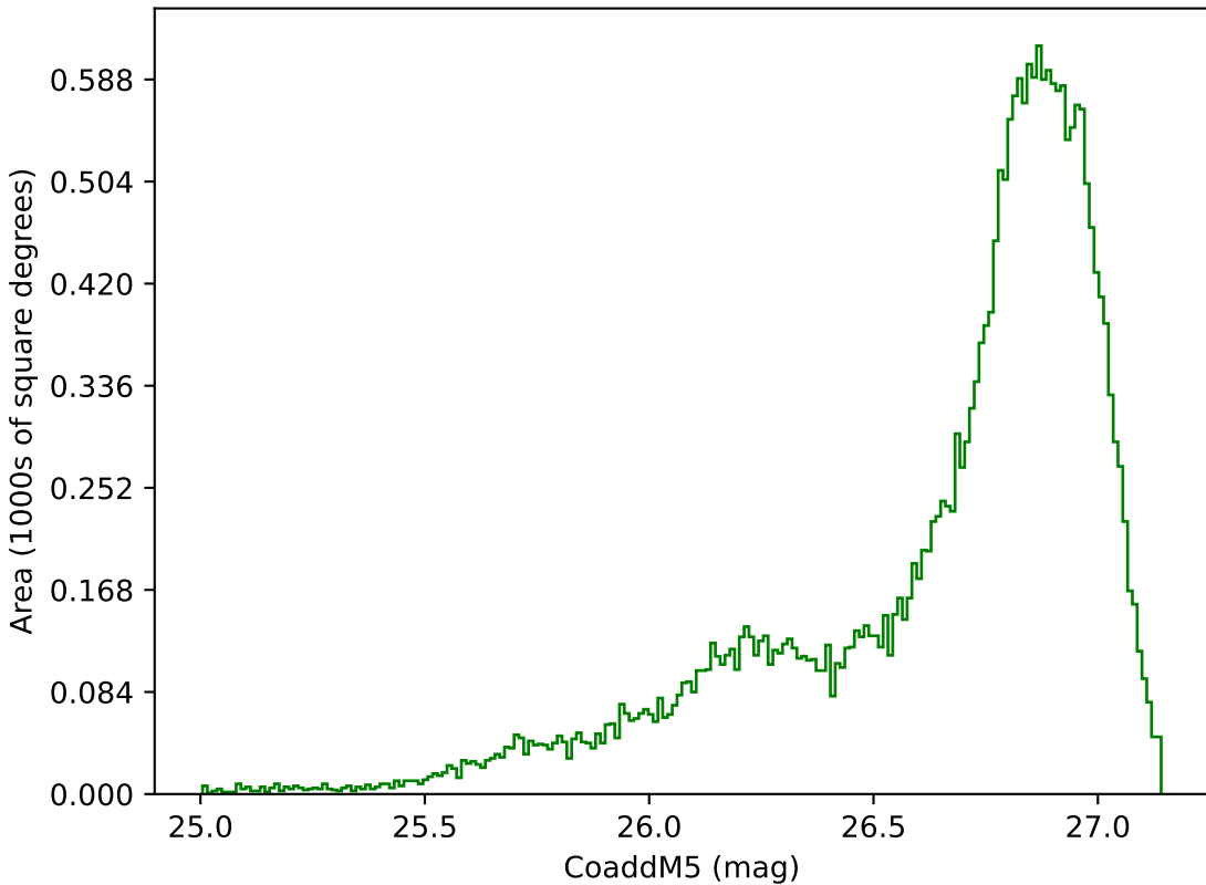
extra_ss_neo3_v3.4_10yrs All sky g band: CoaddM5
