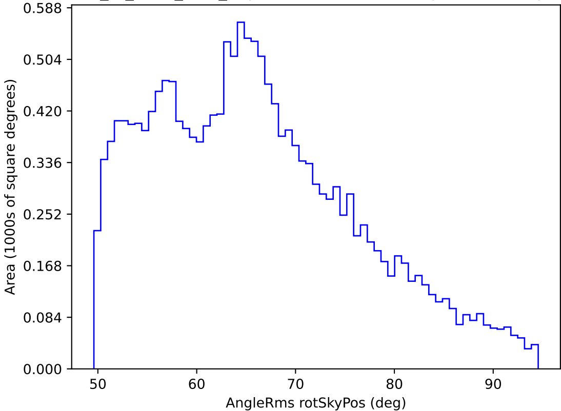
extra_ss_neo3_v3.4_10yrs WFD all bands: AngleRms rotSkyPos
