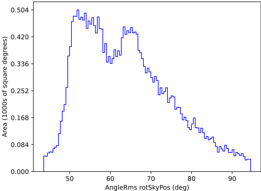
extra_ss_neo3_v3.4_10yrs All sky all bands: AngleRms rotSkyPos
