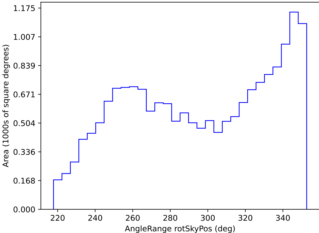
extra_ss_neo3_v3.4_10yrs WFD all bands: AngleRange rotSkyPos
