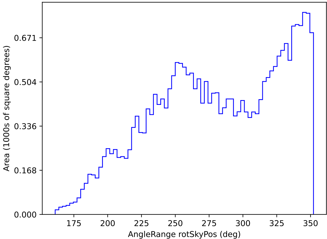
extra_ss_neo3_v3.4_10yrs All sky all bands: AngleRange rotSkyPos
