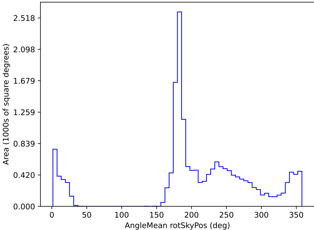
extra_ss_neo3_v3.4_10yrs WFD all bands: AngleMean rotSkyPos
