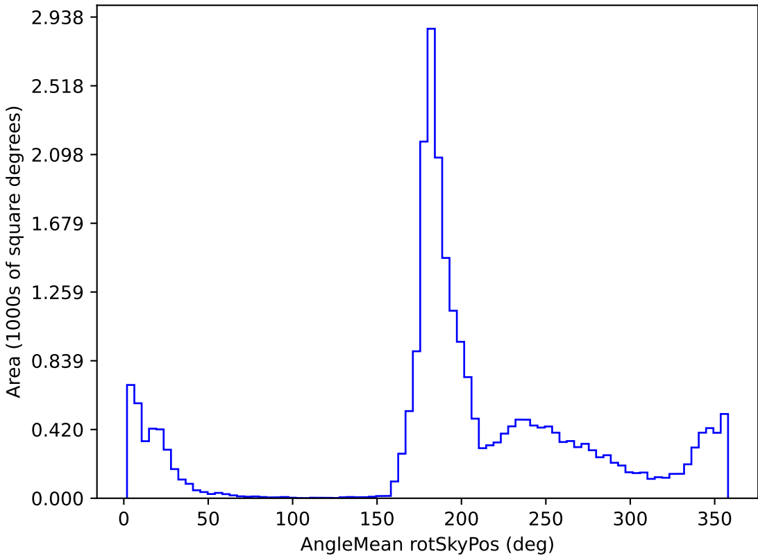
extra_ss_neo3_v3.4_10yrs All sky all bands: AngleMean rotSkyPos
