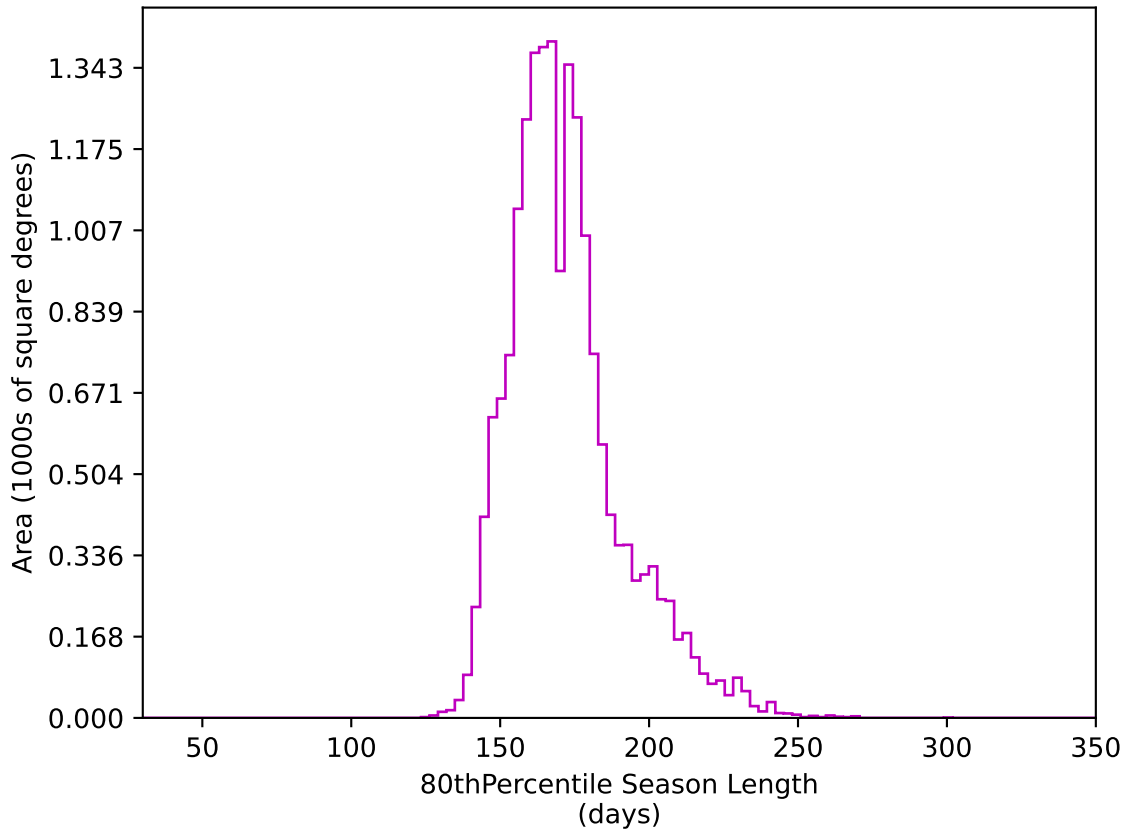
extra_ss_neo3_v3.4_10yrs WFD z band: 80thPercentile Season Length
