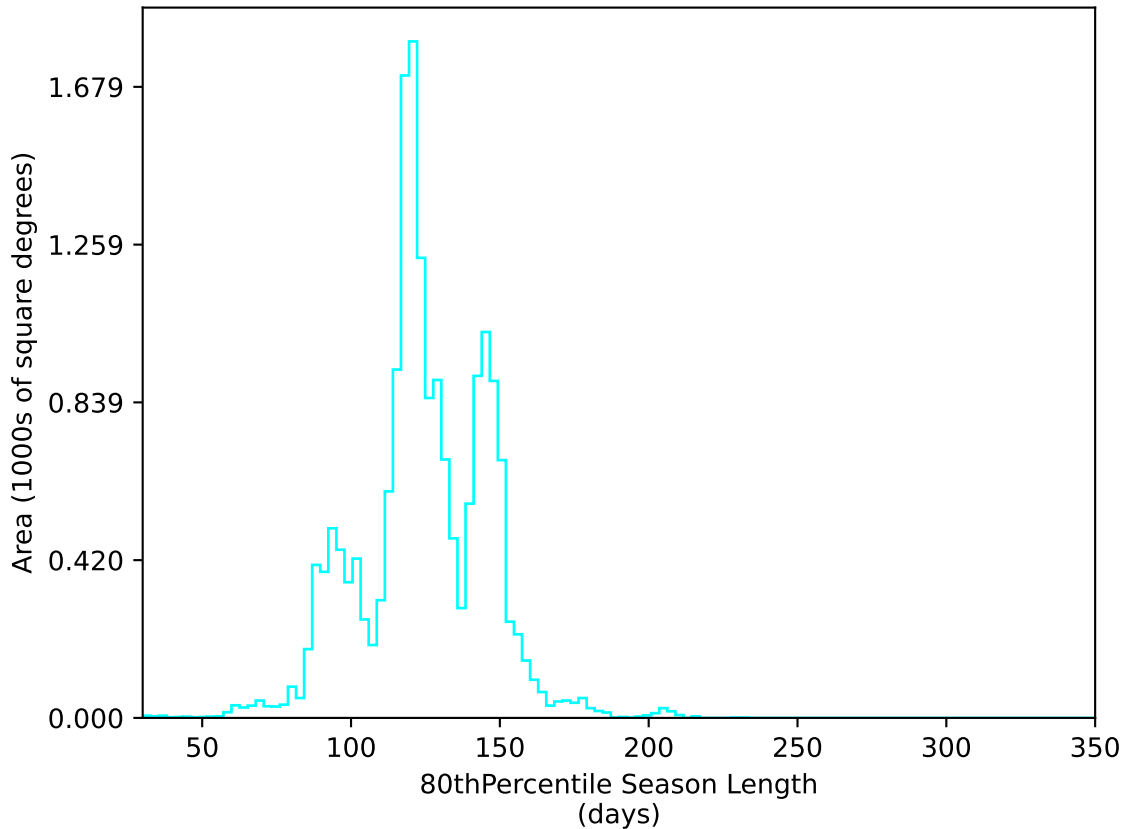
extra_ss_neo3_v3.4_10yrs WFD u band: 80thPercentile Season Length
