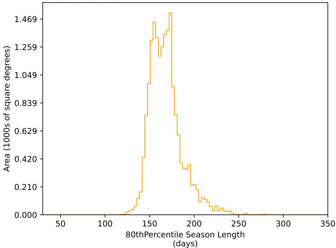
extra_ss_neo3_v3.4_10yrs WFD r band: 80thPercentile Season Length
