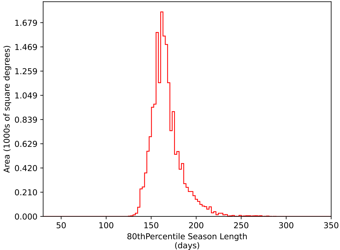
extra_ss_neo3_v3.4_10yrs WFD i band: 80thPercentile Season Length
