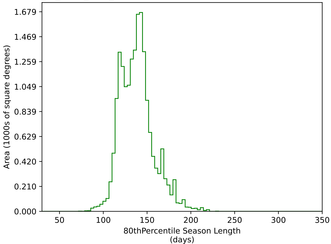
extra_ss_neo3_v3.4_10yrs WFD g band: 80thPercentile Season Length
