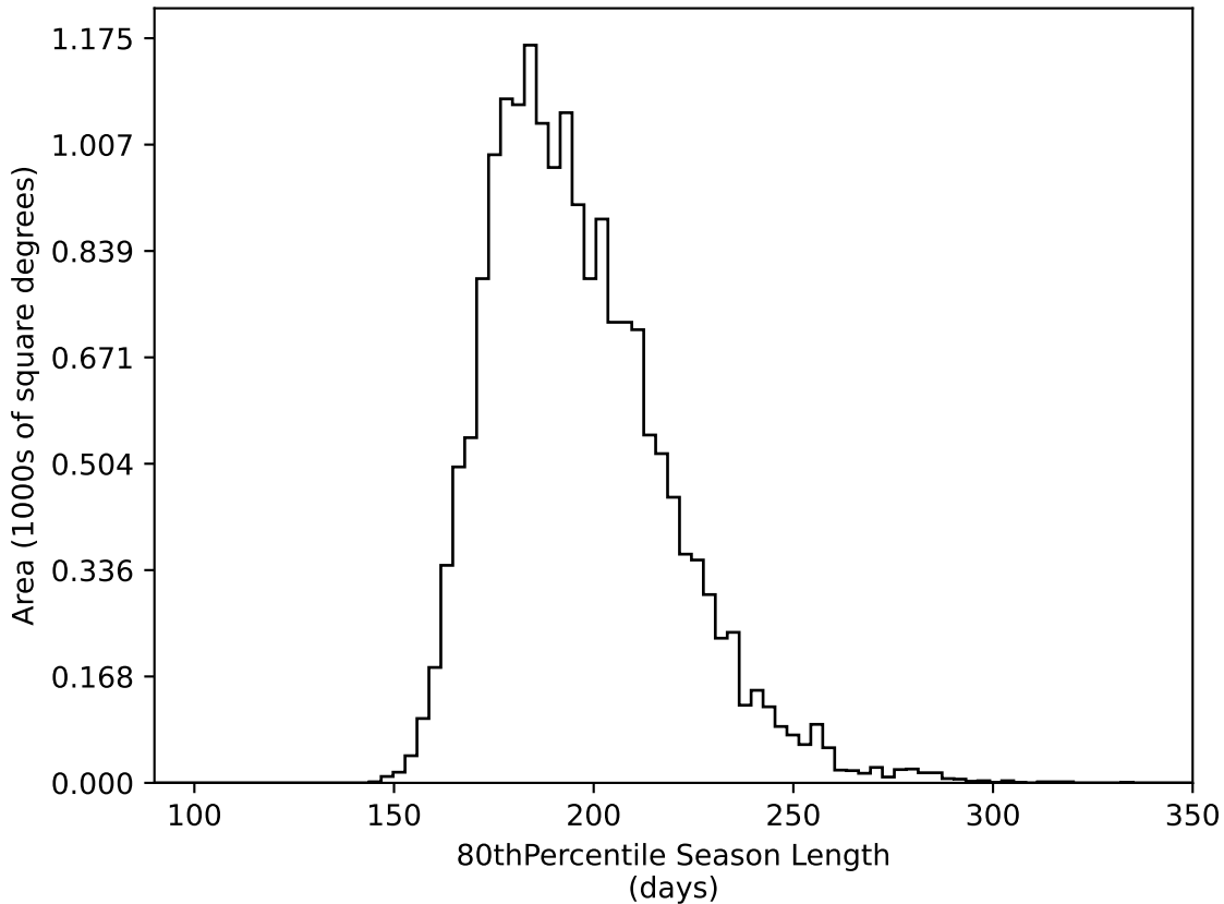
extra_ss_neo3_v3.4_10yrs WFD all bands: 80thPercentile Season Length
