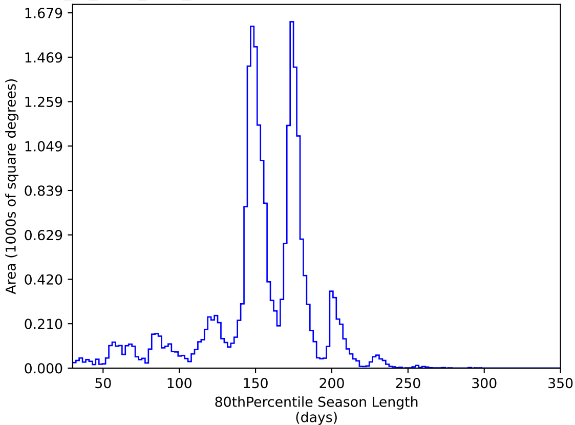
extra_ss_neo3_v3.4_10yrs All sky y band: 80thPercentile Season Length
