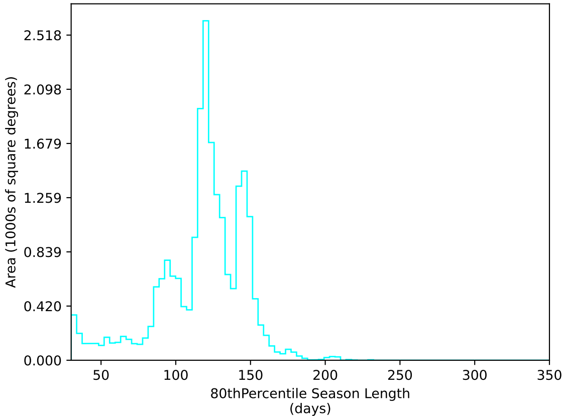
extra_ss_neo3_v3.4_10yrs All sky u band: 80thPercentile Season Length
