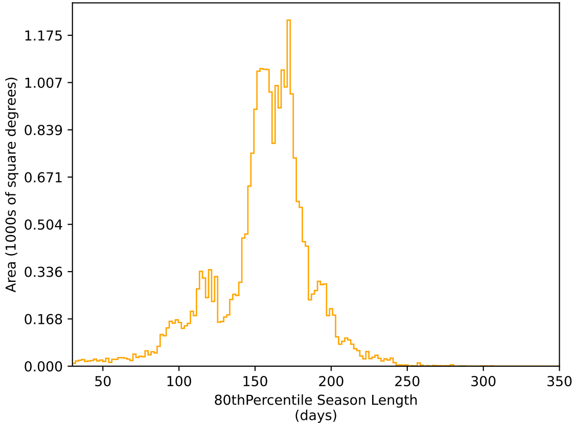
extra_ss_neo3_v3.4_10yrs All sky r band: 80thPercentile Season Length
