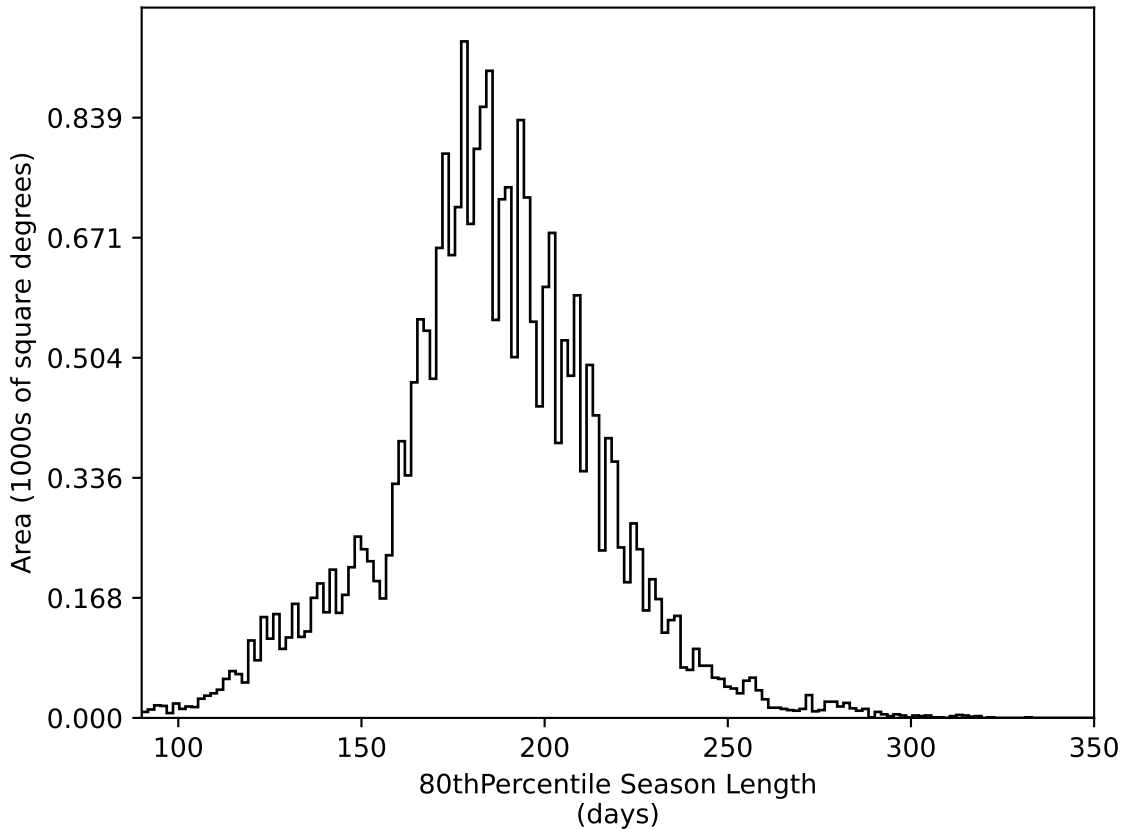
extra_ss_neo3_v3.4_10yrs All sky all bands: 80thPercentile Season Length
