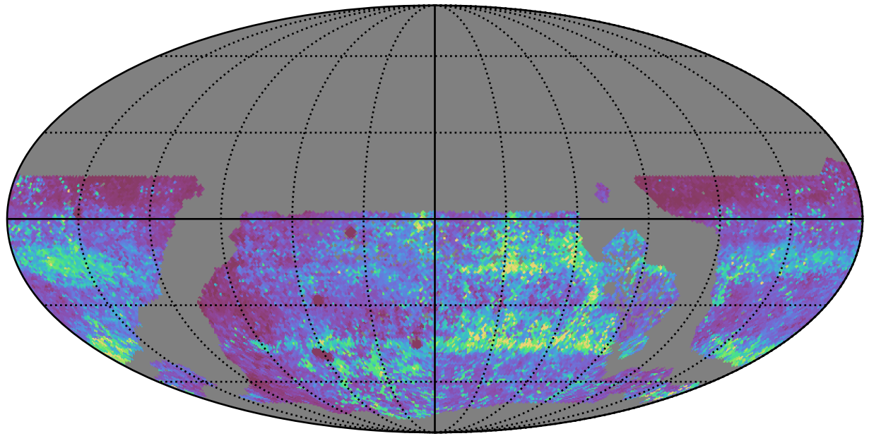
extra_ss_neo3_v3.4_10yrs WFD zy bands: 75th Percentile Intranight Timespan
