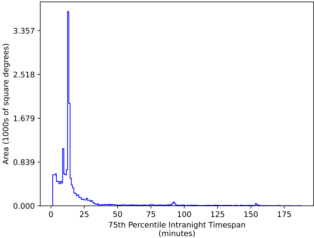
extra_ss_neo3_v3.4_10yrs WFD z band: 75th Percentile Intranight Timespan
